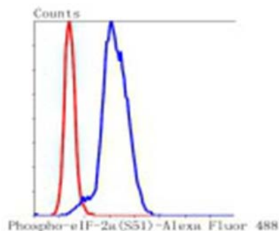
Fig. 3. Flow cytometric analysis of HeLa cells with Phospho-eIF-2a (Ser51) antibody at 1/50 dilution (blue) compared with an unlabelled control (cells without incubation with primary antibody; red). Alexa Fluor 488-conjugated goat anti rabbit IgG was used as the secondary antibody.
